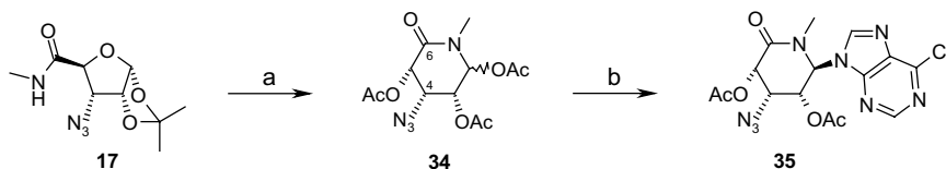
Scheme 3. Reagents and conditions: (a) (i) 70% HOAc, 60 °C; (ii) Ac 2 O–pyridine (1:2), rt; (b) silylated 6-chloropurine, TMSOTf, dry 1,2-dichloroethane, reflux.
